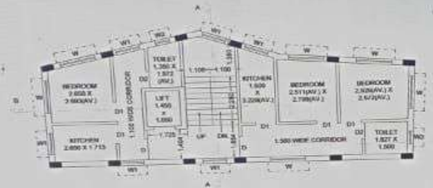
PROPOSED TYPICAL FLOOR PLAN SCALE 1:100
